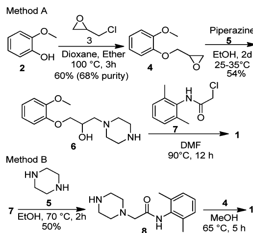
Scheme 1. Precedented synthetic approach (methods A and B)
